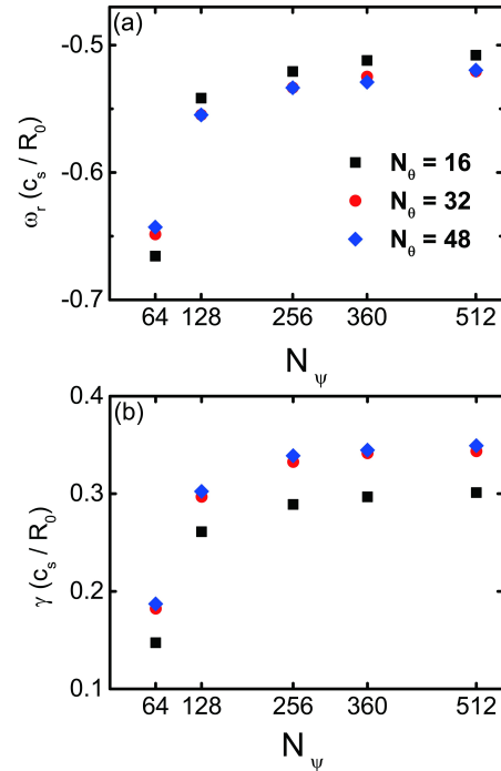
Figure 3. Convergence of (a) real frequency and (b) growth rate on the radial and poloidal grid mesh ( N_\psi, N_\theta ). k_\theta \rho_s = 0.5 , \kappa_{T_i} = 10.47 . The adiabatic electron model is adopted.
