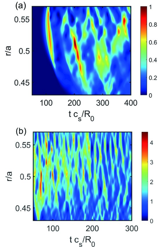
Figure 16. The time-spatial contour structure of the ion heat transport coefficient \chi_i / \chi_{GB} at the nonlinear stage with (a) the adiabatic electron model and (b) the kinetic electron model.
