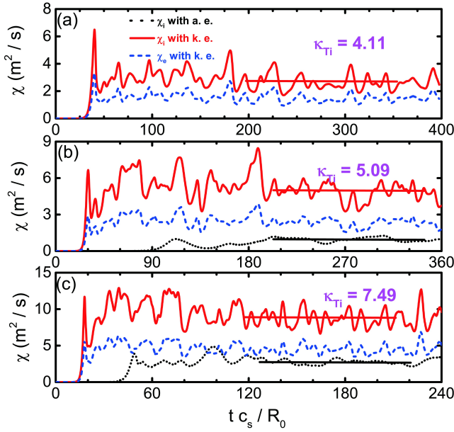
Figure 13. Time evolutions of the heat diffusivities for ions and electrons for \kappa_{Ti} = 4.11 , 5.09 and 7.49 with the adiabatic and kinetic electron models adopted. The horizontal lines are labeled for the time-average range.
