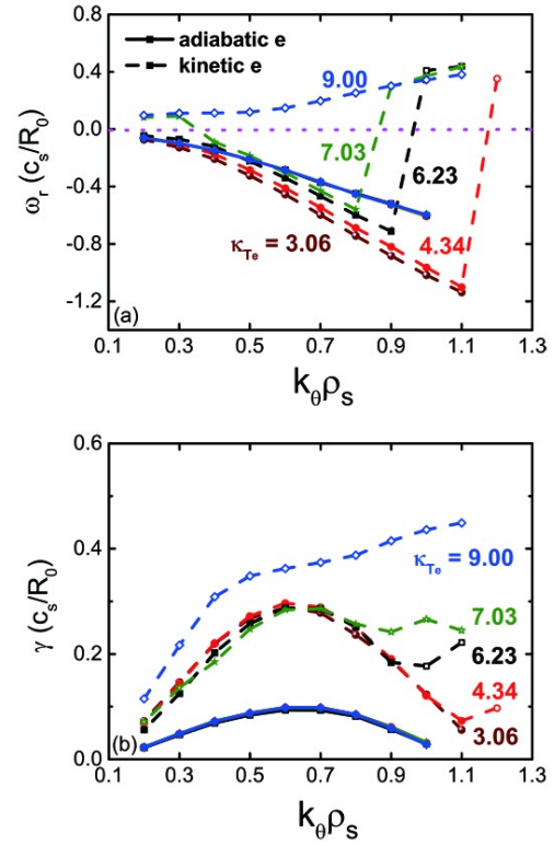
Figure 5. Real frequency (a) and growth rate (b) versus k_{\theta}\rho_s for \kappa_{Te} = 3.06, 4.34, 6.23, 7.03 and 9.00. The solid and dashed lines denote the adiabatic and kinetic electron models, respectively. The magenta dashed line denotes \omega_r = 0 .
