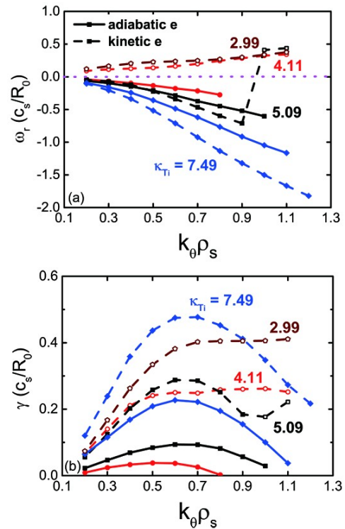
Figure 4. Real frequency (a) and growth rate (b) versus k_{\theta} \rho_s for \kappa_{Ti} = 2.99, 4.11, 5.09 and 7.49 . The solid and dashed lines denote the adiabatic and kinetic electron models, respectively. The magenta dashed line denotes \omega_r = 0 . The negative (solid symbols) and positive (open symbols) real frequencies denote the ITG instability and TEM, respectively.
