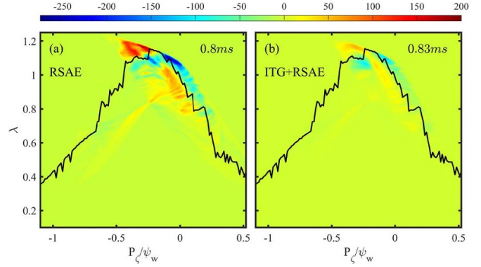
Figure 7. Perturbed EP distribution function \delta f in (P_\zeta, \lambda) phase space with fixed \mu B_a = 80\text{keV} at 0.8ms from single scale RSAE simulation [panel (a)] and at 0.83ms from standard coupled simulation [panel (b)]. The black lines represent the dominant linear resonance.
