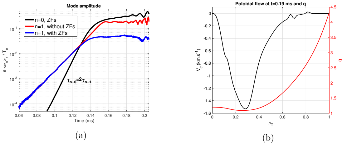
Figure 7: (a) Time evolution of volume-averaged perturbed electrostatic potential e\langle\phi\rangle/T_e ( n=0,1 ). (b) Zonal poloidal flow V_\theta ( \text{km}\cdot\text{s}^{-1} ) after saturation at t=0.19\text{ms} in GTC simulations. Figure (a) is reproduced from [59]
