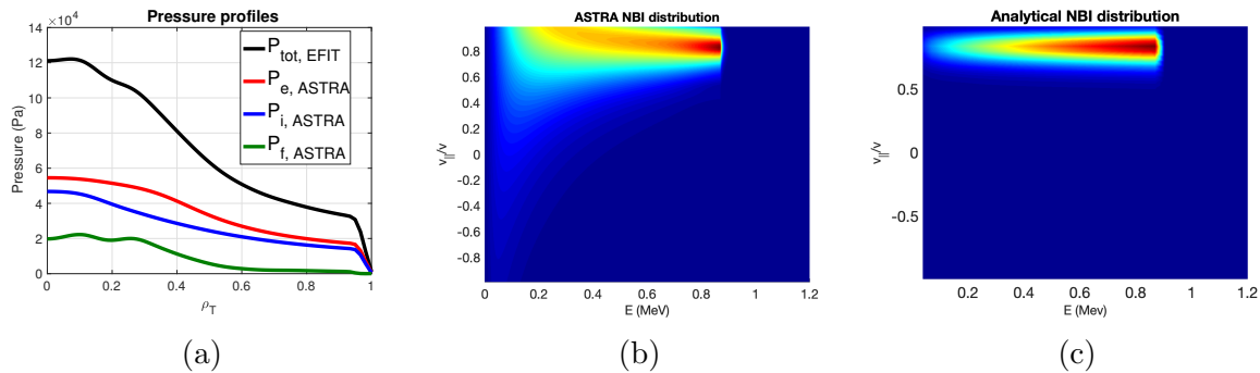
Figure 4: ITER #1001006 numerical equilibrium at t=1580\text{ms} . (a) Partial pressure profiles (b) ASTRA and (c) analytical NBI distributions in the (E, v_{||}/v) phase space diagram.
