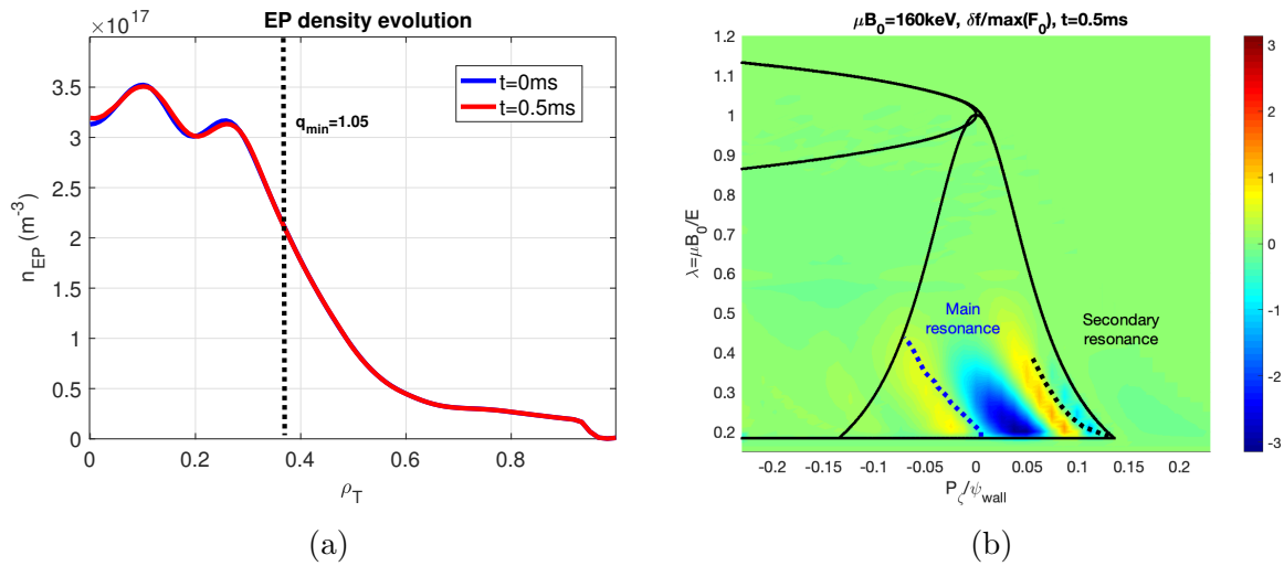
Figure 15: (a) EP density profile before and after fishbone burst without zonal flows. (b) Perturbed distribution function in (P_\zeta, \lambda) CoM phase space at \mu B_0 = 160keV .
