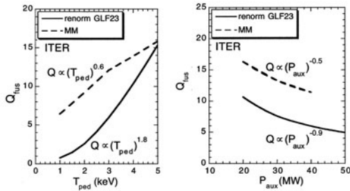
Fig. III.3.1 ITER performance Q projection vs T_{\text{ped}} at P_{\text{aux}}=40 MW (a) and vs P_{\text{aux}} at T_{\text{ped}}=3 keV (b). The “renormed GLF23” model has an 8.3% RMS deviation to 50 H-mode DIII-D, JET, CMod discharges. From [Kinsey 2003]
