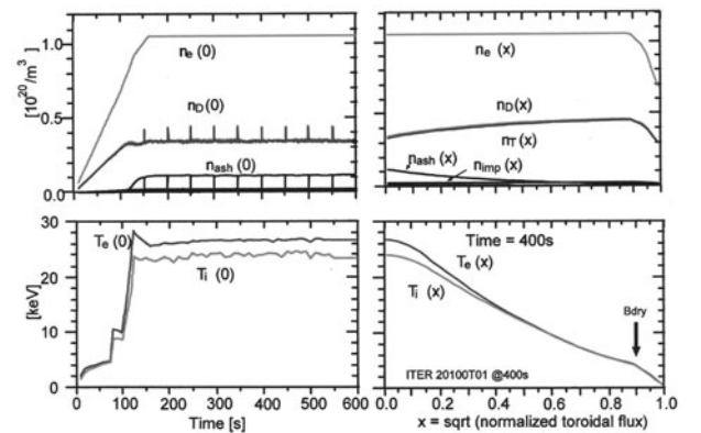
Fig. III.9.1 (a, b) Temperatures and (c, d) densities in an ITER H-mode plasma
