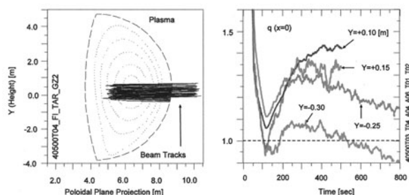
Fig.III.9.6 a) Samples of NNBI neutral 3D trajectories into sections at their toroidal angle; b) calculated q(0) in a ITER hybrid plasma (with high \beta_n ) with varying height Y of the peak neutral flux at the tangency radius measured from the vessel midplane, indicating that q(0) can be maintained above unity for long durations
