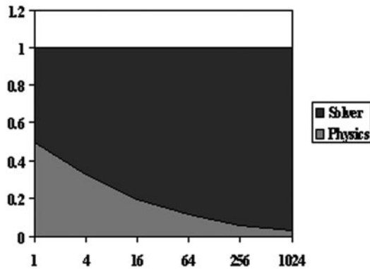
Fig.V.1.1 Fraction of time spent in the solver and in the physics phases of a typical PDE simulation as the problem is scaled by a factor of one thousand, assuming that the computation is originally well balanced on one processor and that the complexity of the solver phase grows like the 3/2 ths power of the discretization size, whereas the physics phase grows linearly
