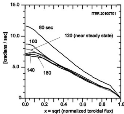
Fig.III.9.4 Profile of toroidal rotation in an ITER H-mode resulting from the NNBI torque and the transport assumption \chi_{\text{momentum}} = \chi_{\text{ion}}
