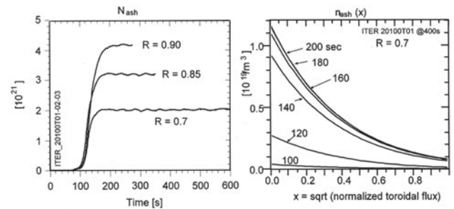
Fig.III.9.5 Simulation of ash from thermalized fusion alpha particles. a) Total number of He ash atoms with assumed values for D and V and three choices of the recycling coefficient; b) ash profiles for 0.7
