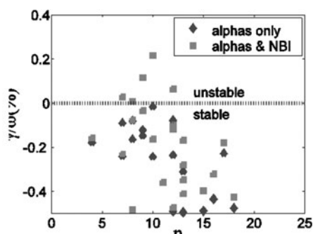
Fig.III.9.7 Computed linear TAE stability versus toroidal mode number n with and without NNBI
