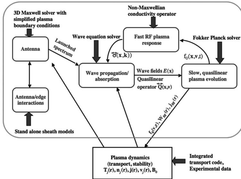
Fig. III.6.1 Elements of an integrated simulation of wave interactions with fusion plasmas
